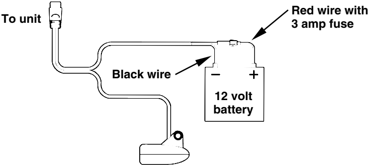
Power connections for the FishEasy 2 family sonar units (direct battery connection shown).
